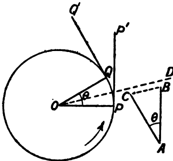
FIG. 31.—LINEAR VELOCITY
